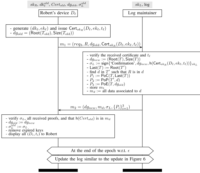
Fig. 8. The protocol for updating keys. In the protocol, dk_\ell^{old} is the current valid ephemeral secret key, \text{Cert}_{old} is the corresponding certificate, dg_{old} and \sigma_L^{old} are the digest and signature received from the log maintainer in the last session, respectively.
