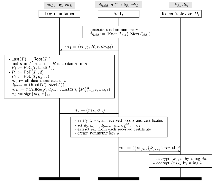
Fig. 7. The protocol for sending and receiving a message. In which, \sigma_L^{old} is the signature received from the log maintainer in the last session. If any of the stated verification checks fails, the agent aborts the protocol.
